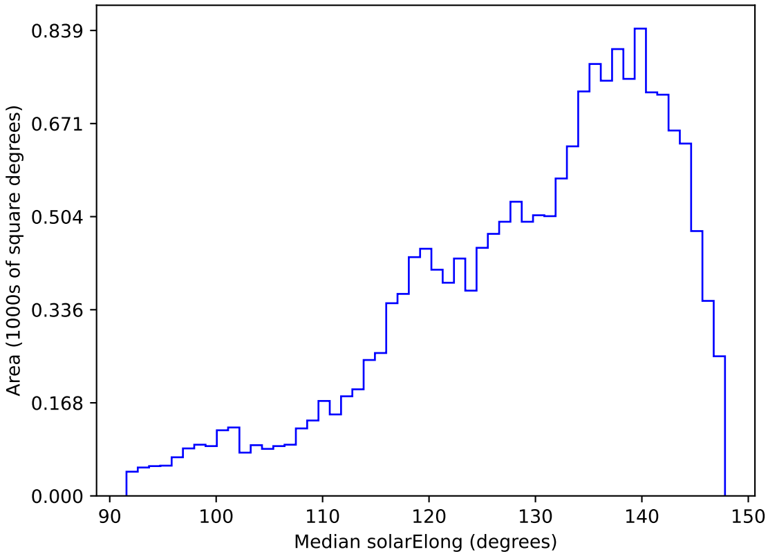
weather_cloudso16v3.4_10yrs WFD i band: Median solarElong
