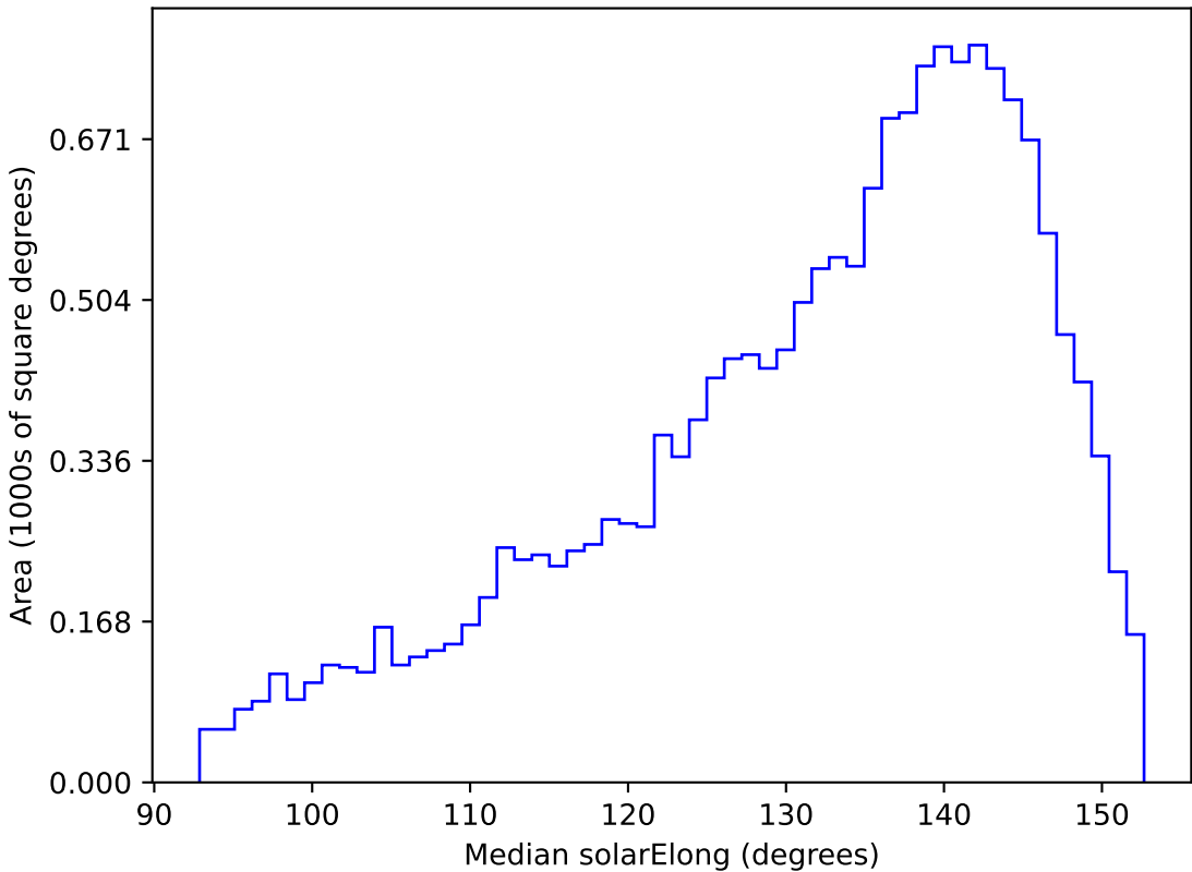
weather_cloudso16v3.4_10yrs WFD g band: Median solarElong
