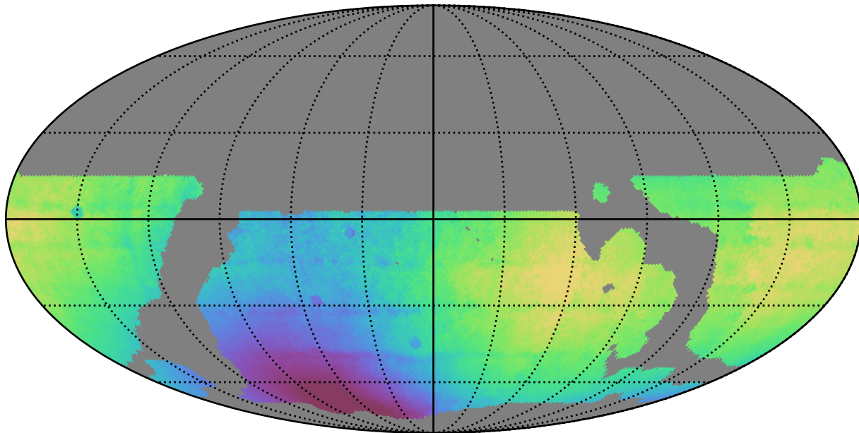
weather_cloudso16v3.4_10yrs WFD all bands: Median solarElong
