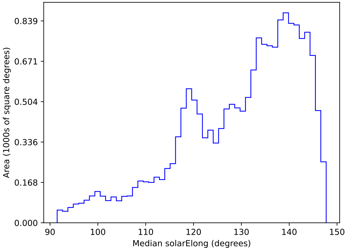
weather_cloudso16v3.4_10yrs WFD all bands: Median solarElong
