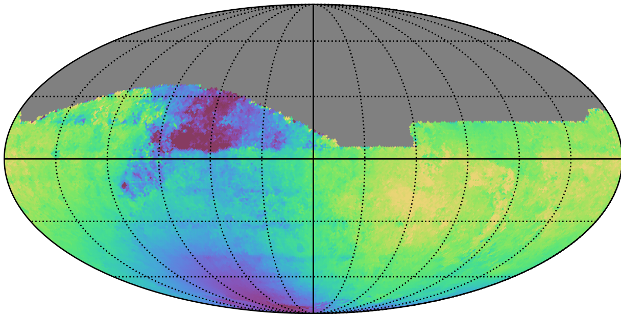
weather_cloudso16v3.4_10yrs All sky z band: Median solarElong
