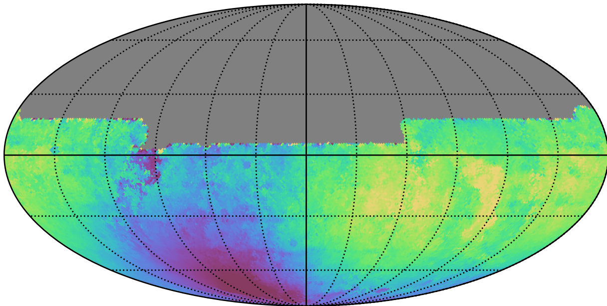
weather_cloudso16v3.4_10yrs All sky y band: Median solarElong
