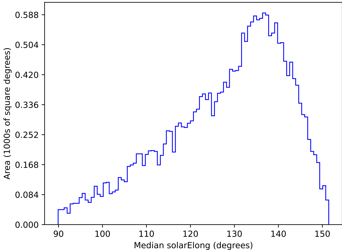
weather_cloudso16v3.4_10yrs All sky y band: Median solarElong
