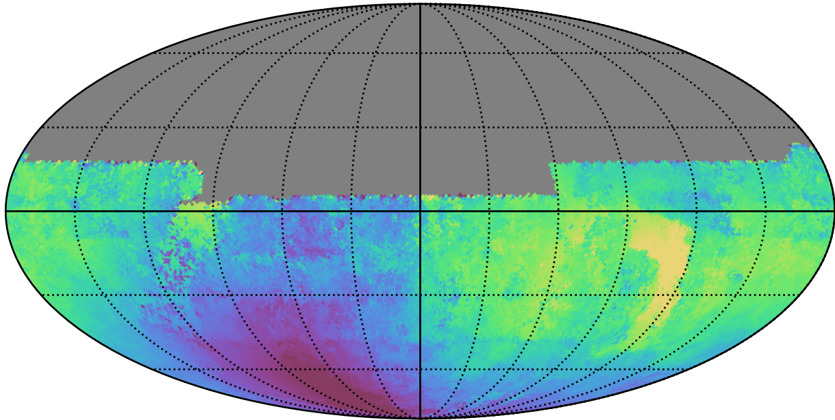
weather_cloudso16v3.4_10yrs All sky u band: Median solarElong
