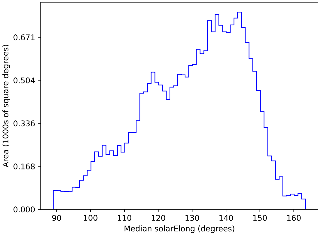
weather_cloudso16v3.4_10yrs All sky u band: Median solarElong
