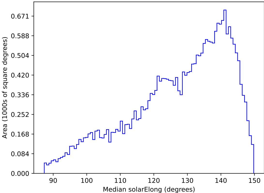
weather_cloudso16v3.4_10yrs All sky r band: Median solarElong
