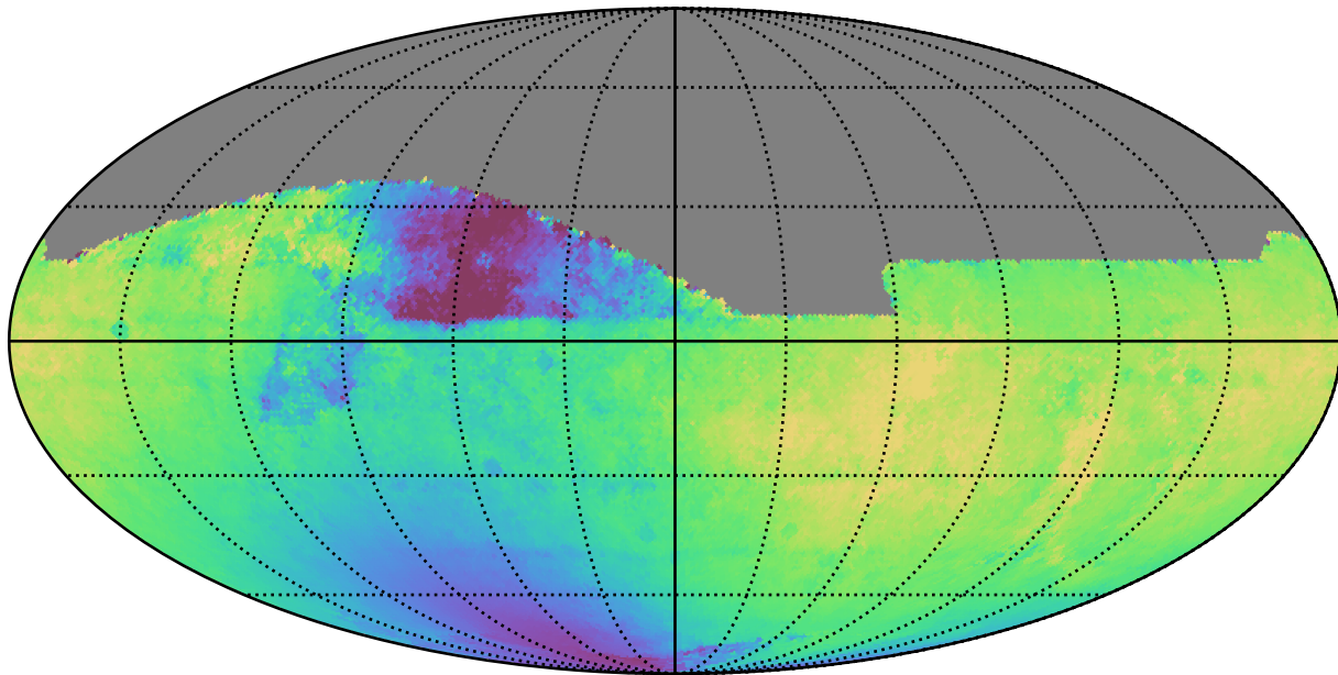
weather_cloudso16v3.4_10yrs All sky i band: Median solarElong
