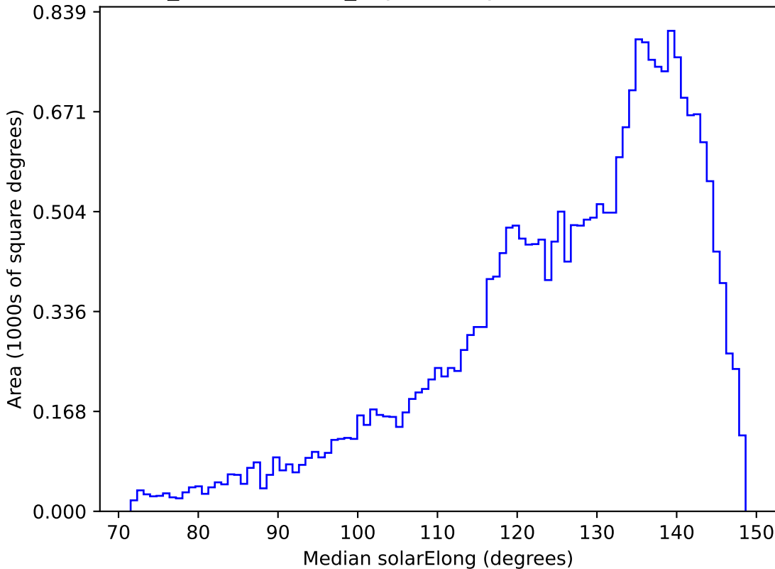
weather_cloudso16v3.4_10yrs All sky i band: Median solarElong
