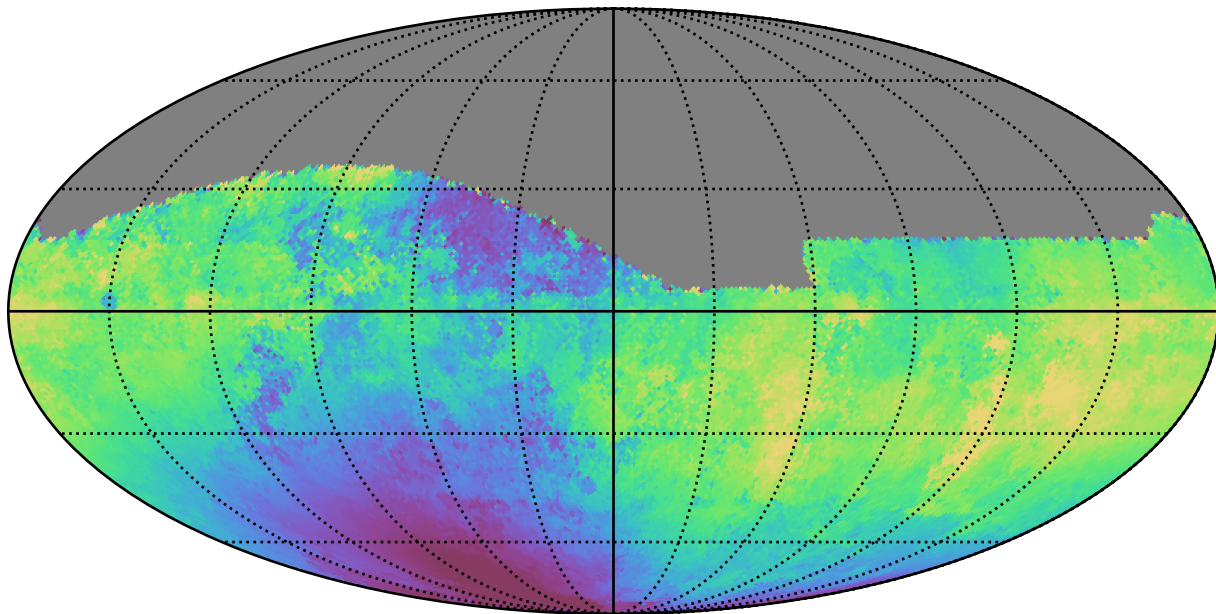
weather_cloudso16v3.4_10yrs All sky g band: Median solarElong
