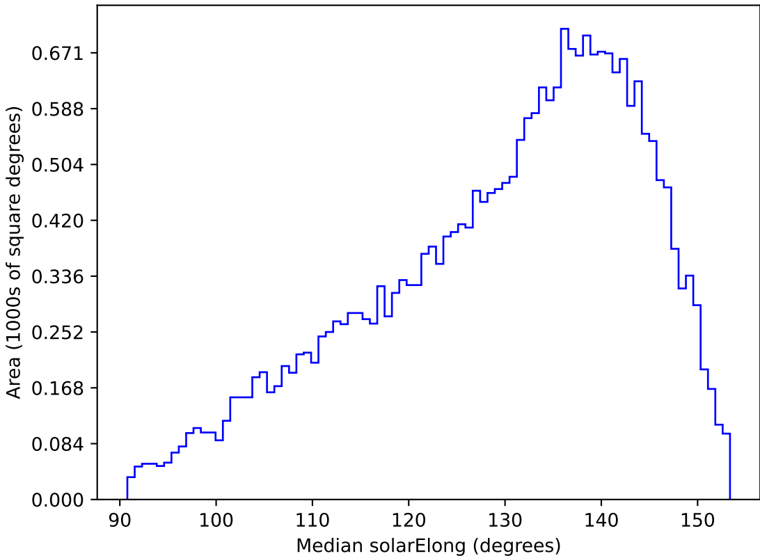
weather_cloudso16v3.4_10yrs All sky g band: Median solarElong
