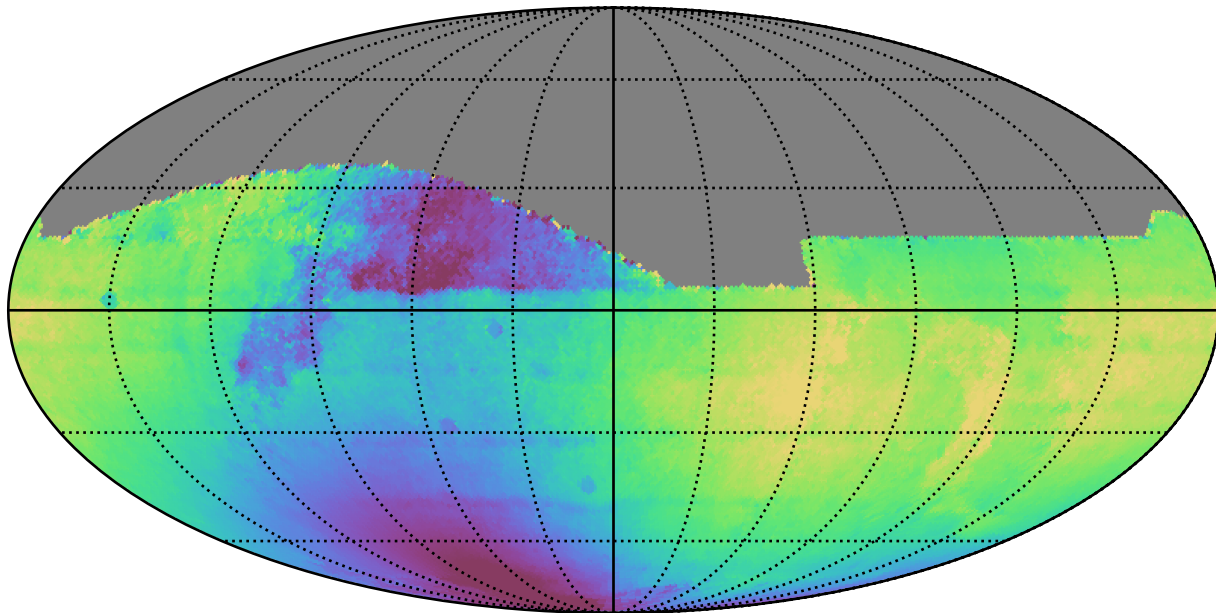
weather_cloudso16v3.4_10yrs All sky all bands: Median solarElong
