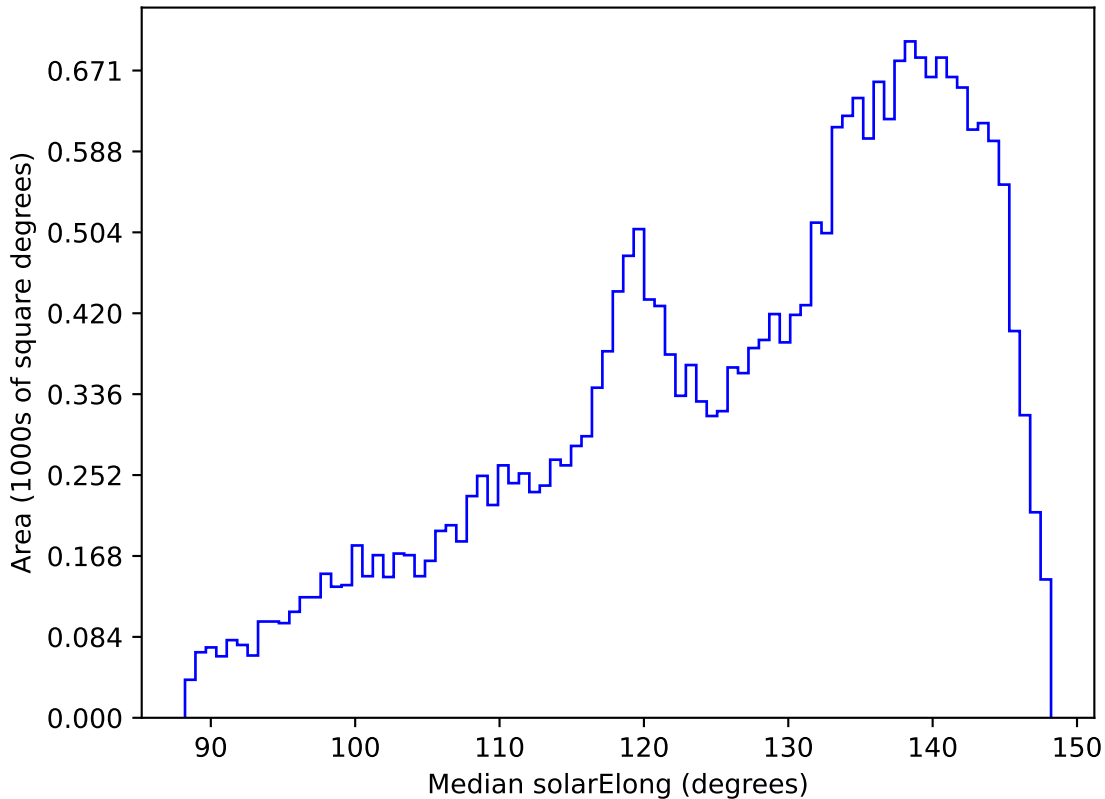
weather_cloudso16v3.4_10yrs All sky all bands: Median solarElong
