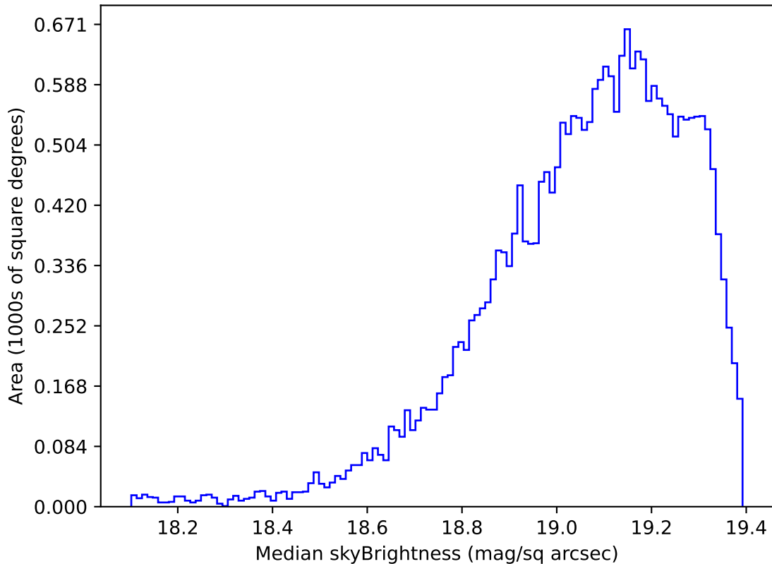
weather_cloudso16v3.4_10yrs Yr 1 z band: Median skyBrightness
