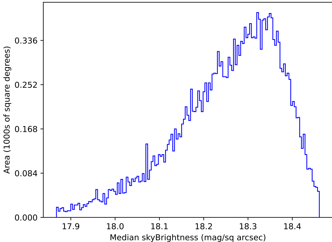
weather_cloudso16v3.4_10yrs Yr 1 y band: Median skyBrightness
