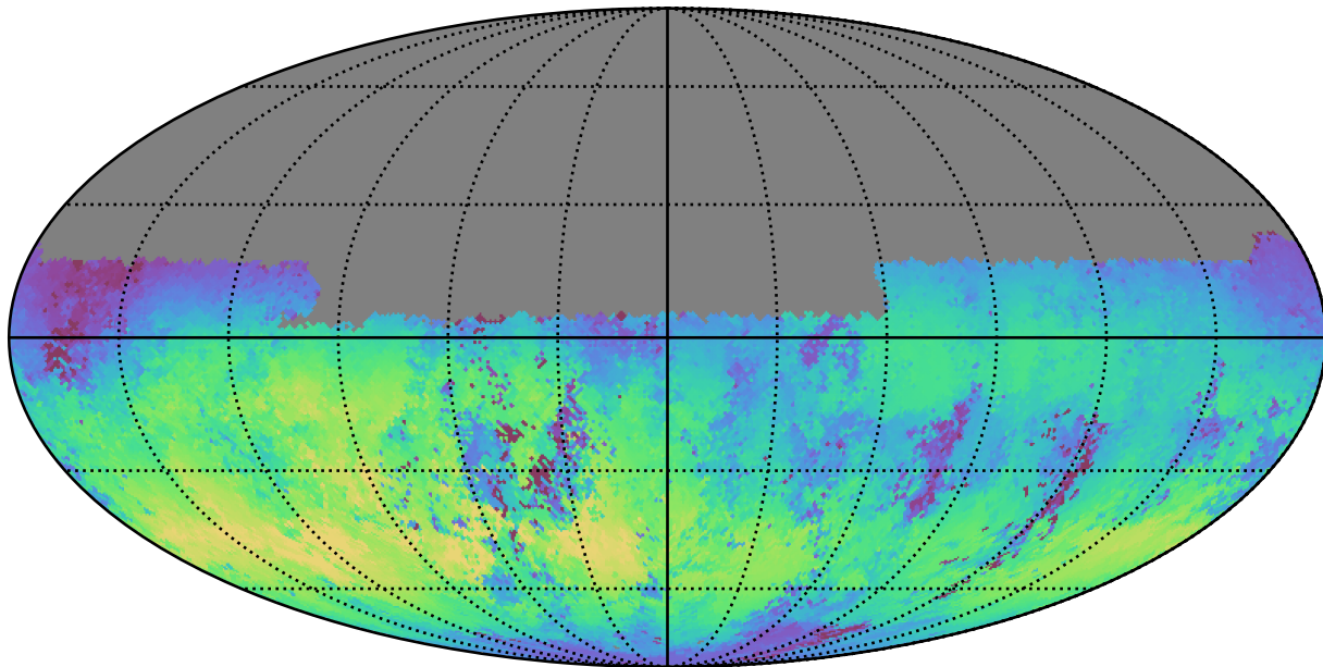
weather_cloudso16v3.4_10yrs Yr 1 u band: Median skyBrightness
