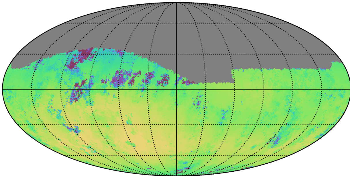
weather_cloudso16v3.4_10yrs Yr 1 r band: Median skyBrightness
