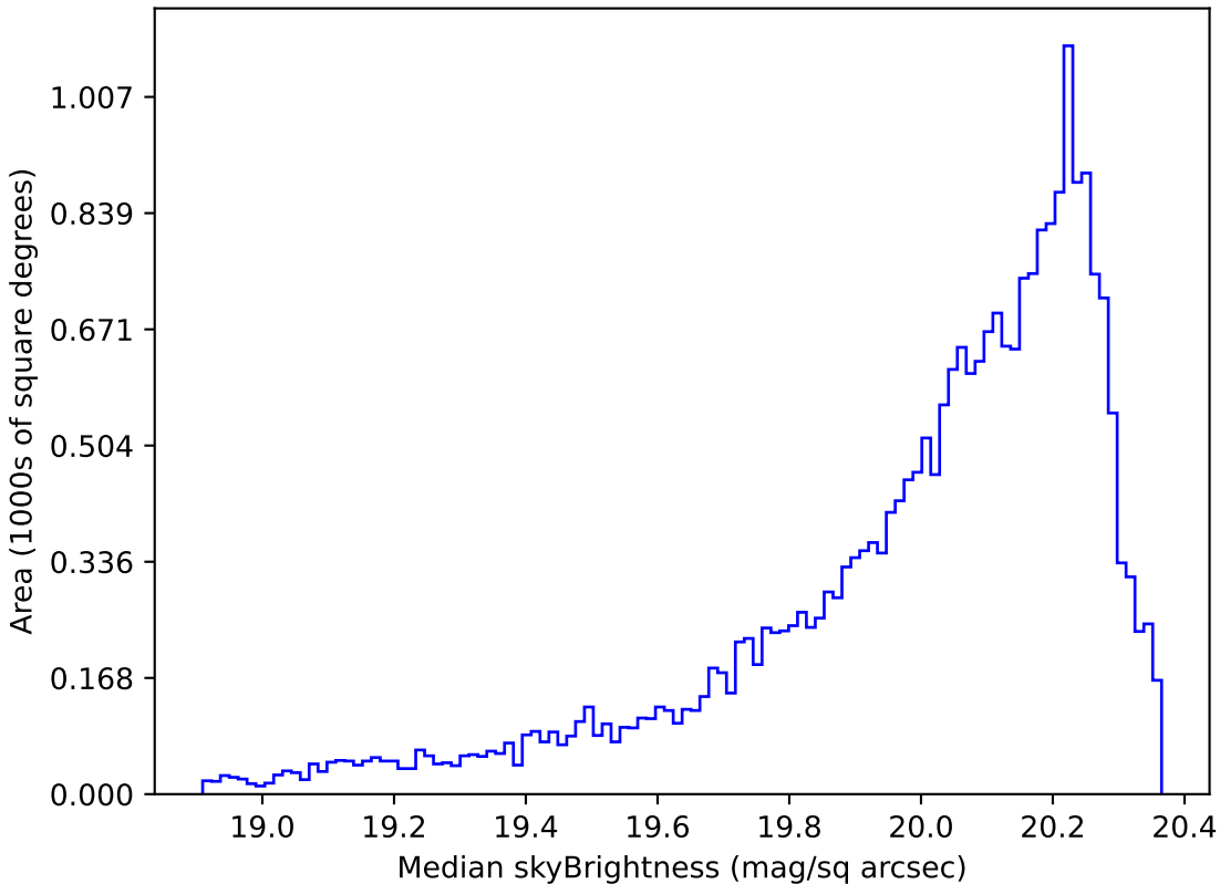
weather_cloudso16v3.4_10yrs Yr 1 i band: Median skyBrightness
