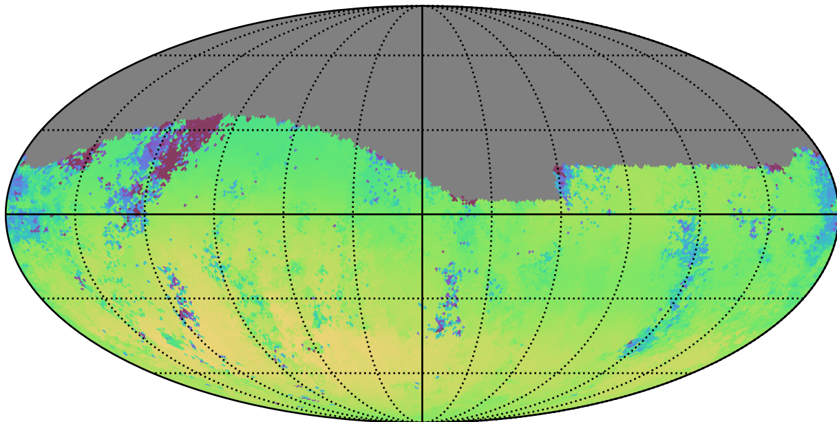
weather_cloudso16v3.4_10yrs Yr 1 g band: Median skyBrightness
