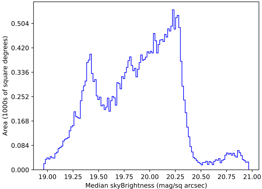
weather_cloudso16v3.4_10yrs Yr 1 all bands: Median skyBrightness
