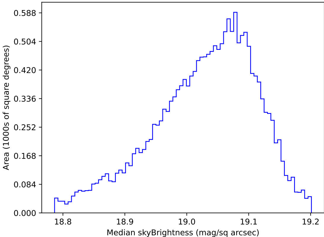
weather_cloudso16v3.4_10yrs WFD z band: Median skyBrightness
