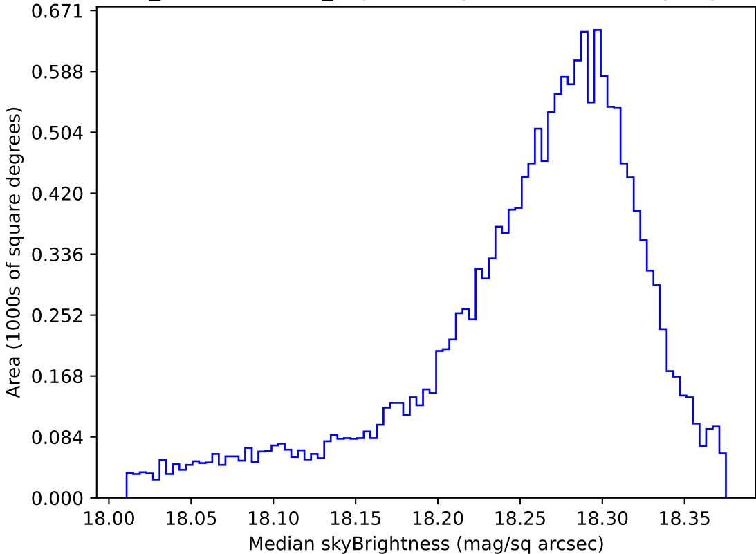
weather_cloudso16v3.4_10yrs WFD y band: Median skyBrightness
