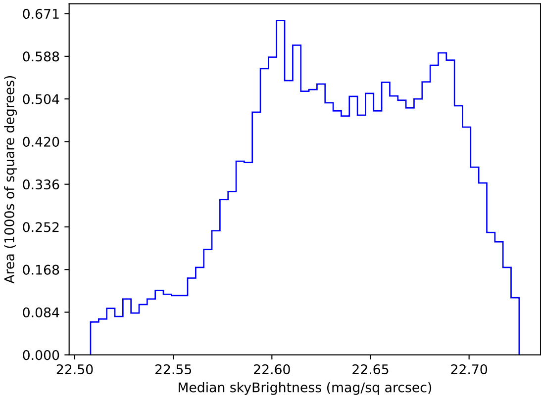
weather_cloudso16v3.4_10yrs WFD u band: Median skyBrightness
