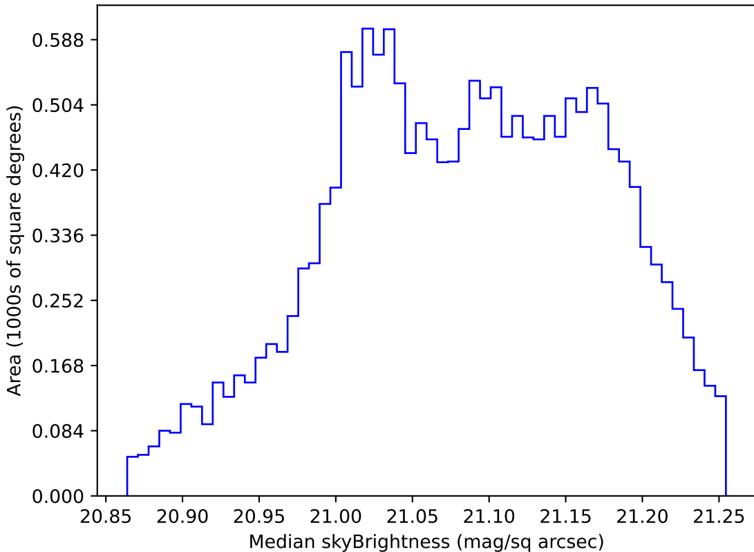
weather_cloudso16v3.4_10yrs WFD r band: Median skyBrightness
