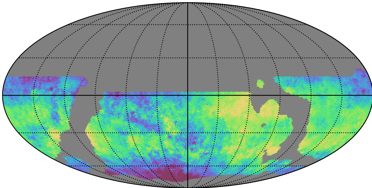
weather_cloudso16v3.4_10yrs WFD i band: Median skyBrightness
