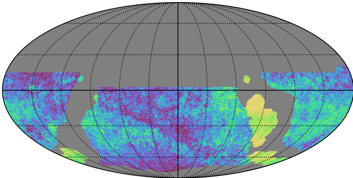
weather_cloudso16v3.4_10yrs WFD all bands: Median skyBrightness
