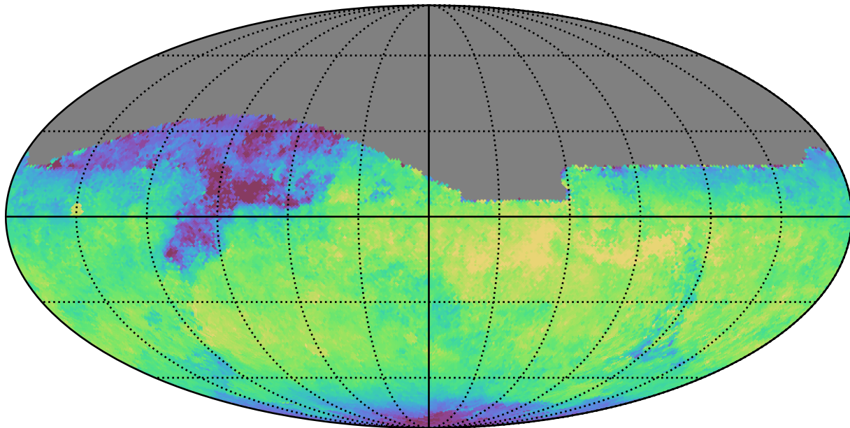
weather_cloudso16v3.4_10yrs All sky z band: Median skyBrightness
