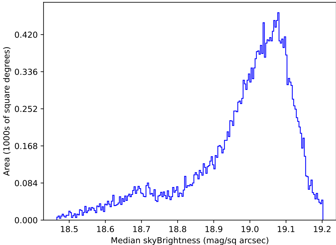
weather_cloudso16v3.4_10yrs All sky z band: Median skyBrightness
