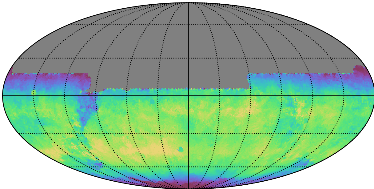
weather_cloudso16v3.4_10yrs All sky y band: Median skyBrightness
