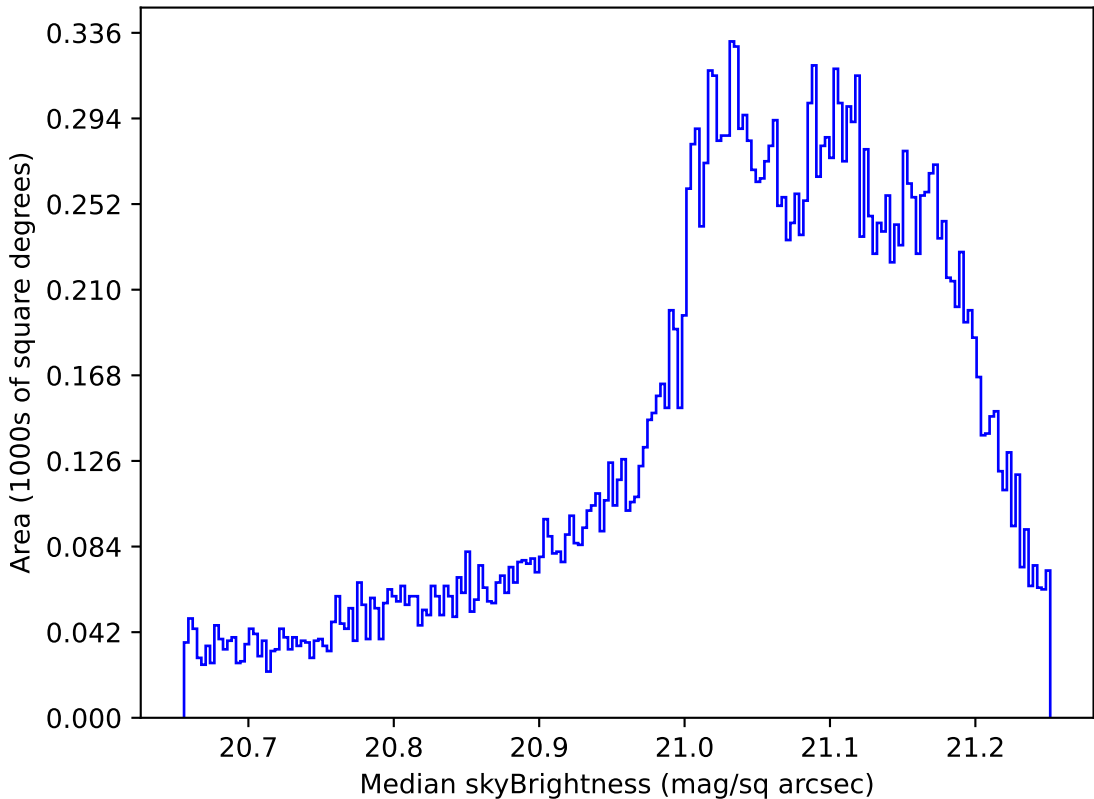
weather_cloudso16v3.4_10yrs All sky r band: Median skyBrightness
