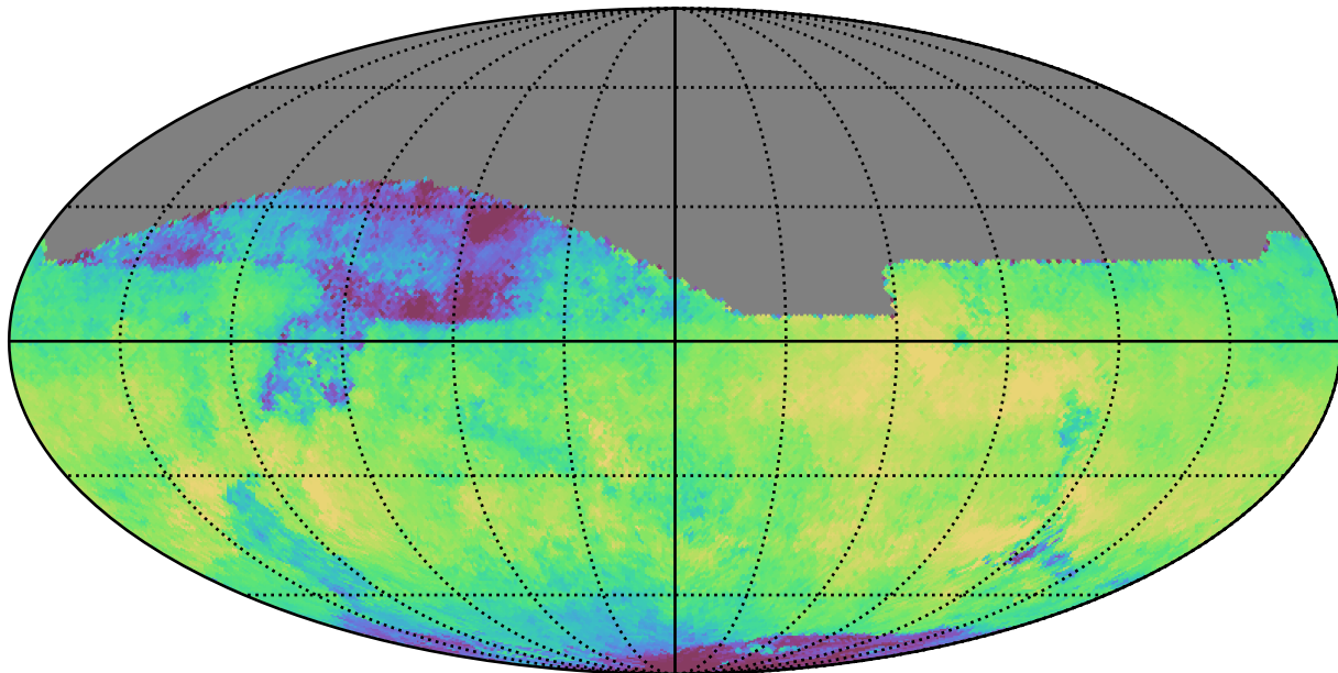
weather_cloudso16v3.4_10yrs All sky i band: Median skyBrightness
