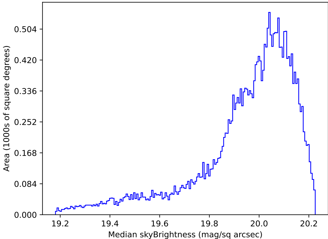
weather_cloudso16v3.4_10yrs All sky i band: Median skyBrightness
