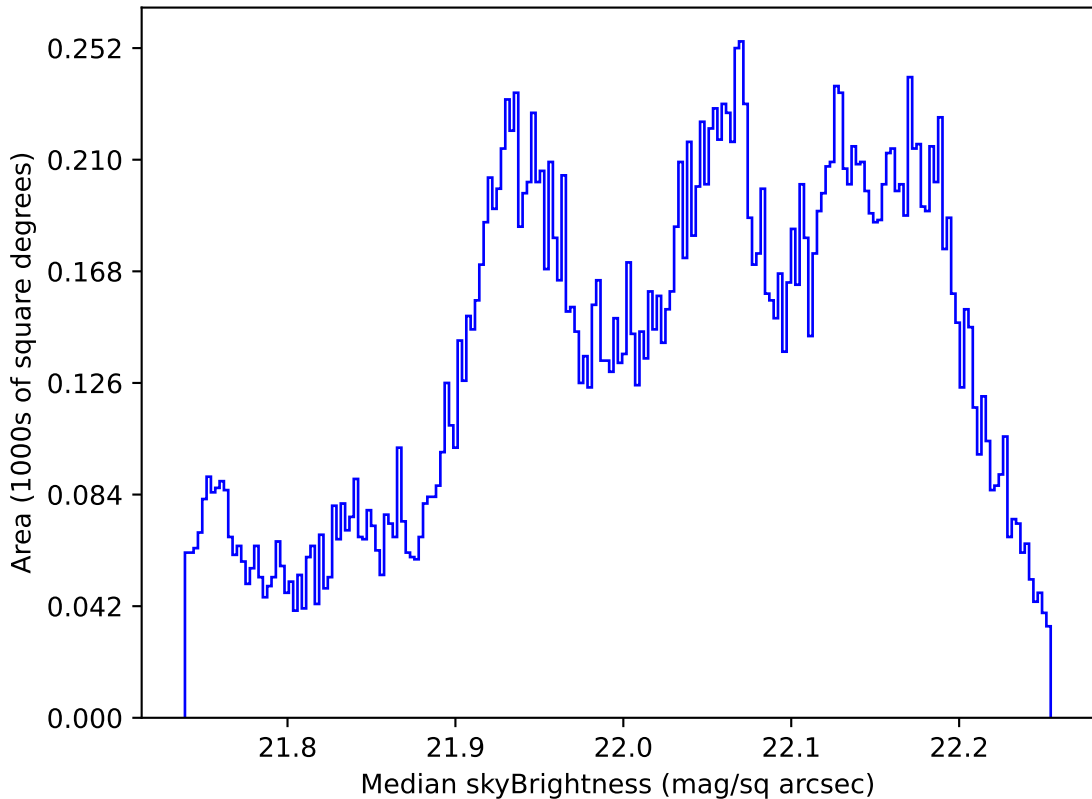
weather_cloudso16v3.4_10yrs All sky g band: Median skyBrightness
