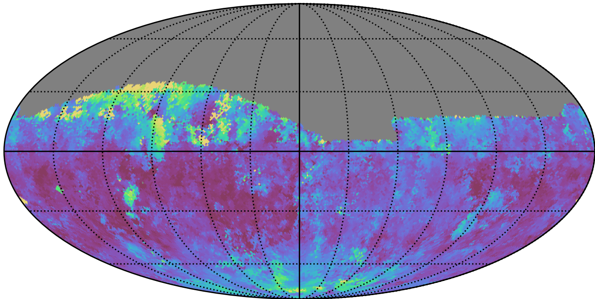
weather_cloudso16v3.4_10yrs Yr 1 z band: Median seeingGeom
