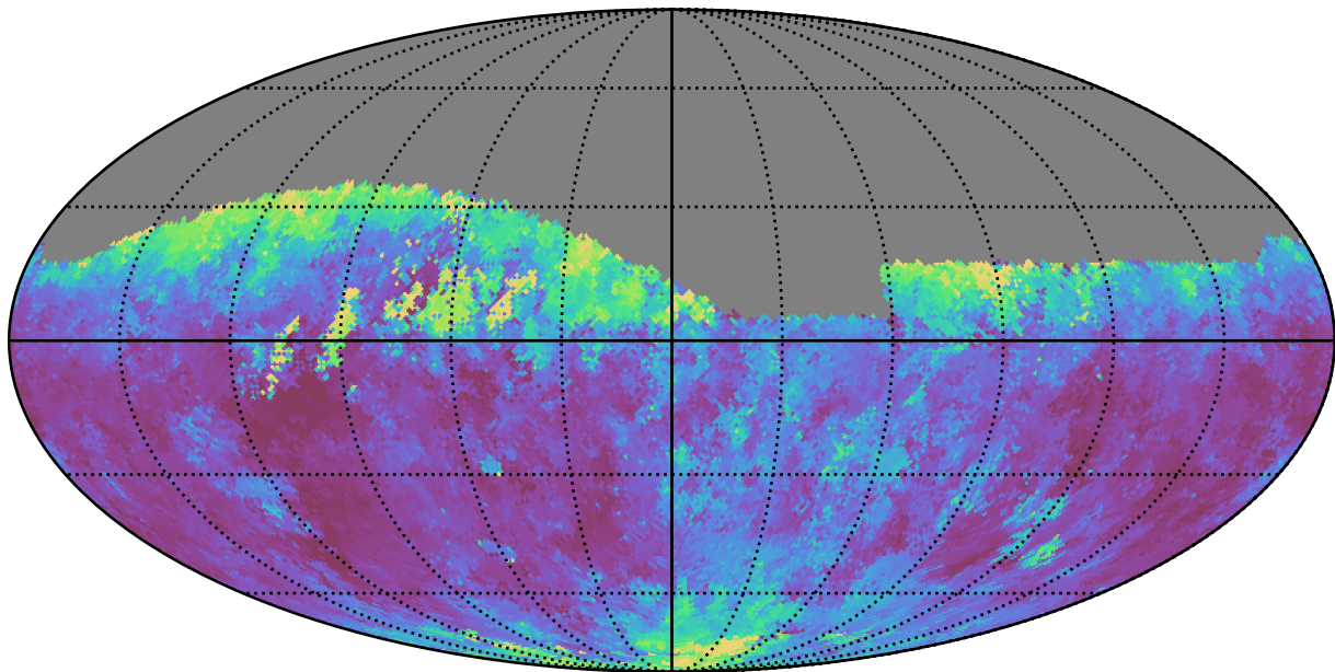
weather_cloudso16v3.4_10yrs Yr 1 r band: Median seeingGeom
