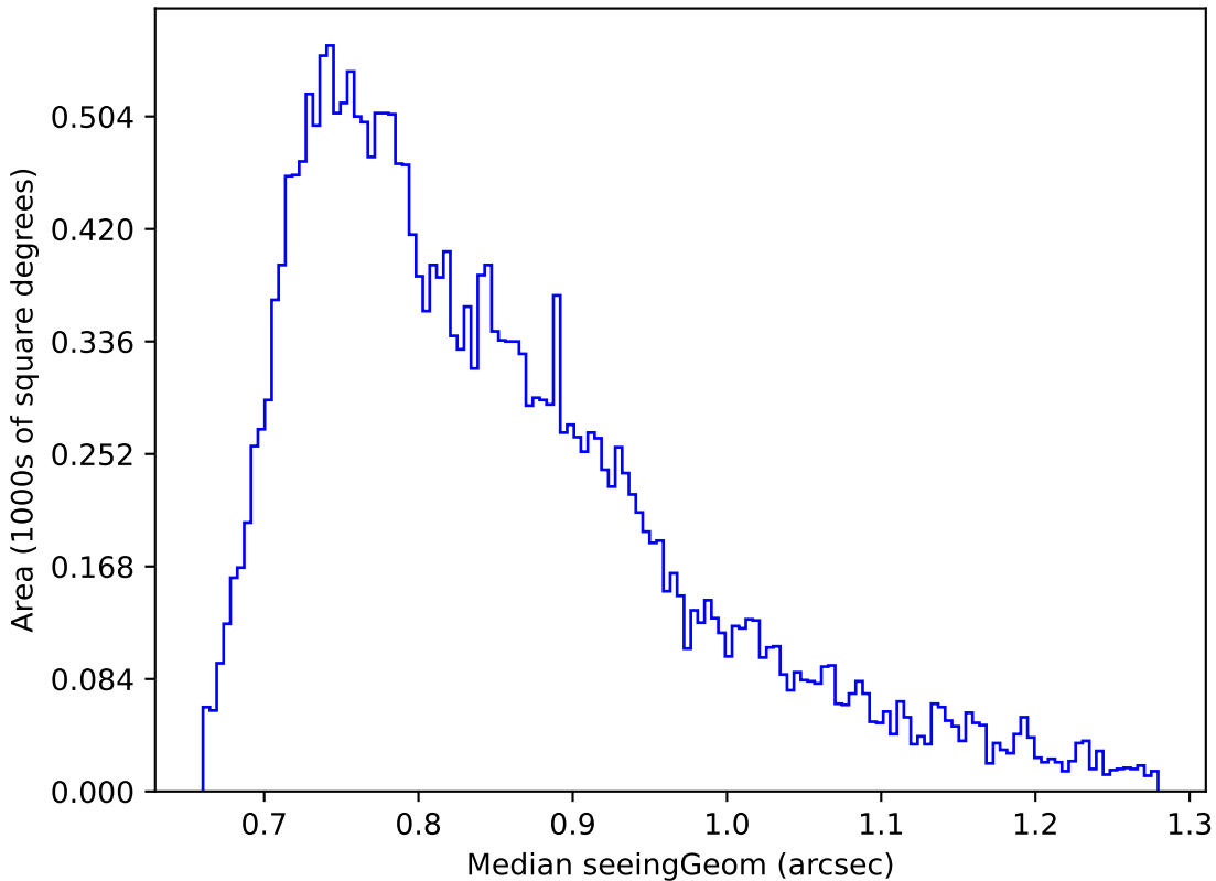
weather_cloudso16v3.4_10yrs Yr 1 r band: Median seeingGeom
