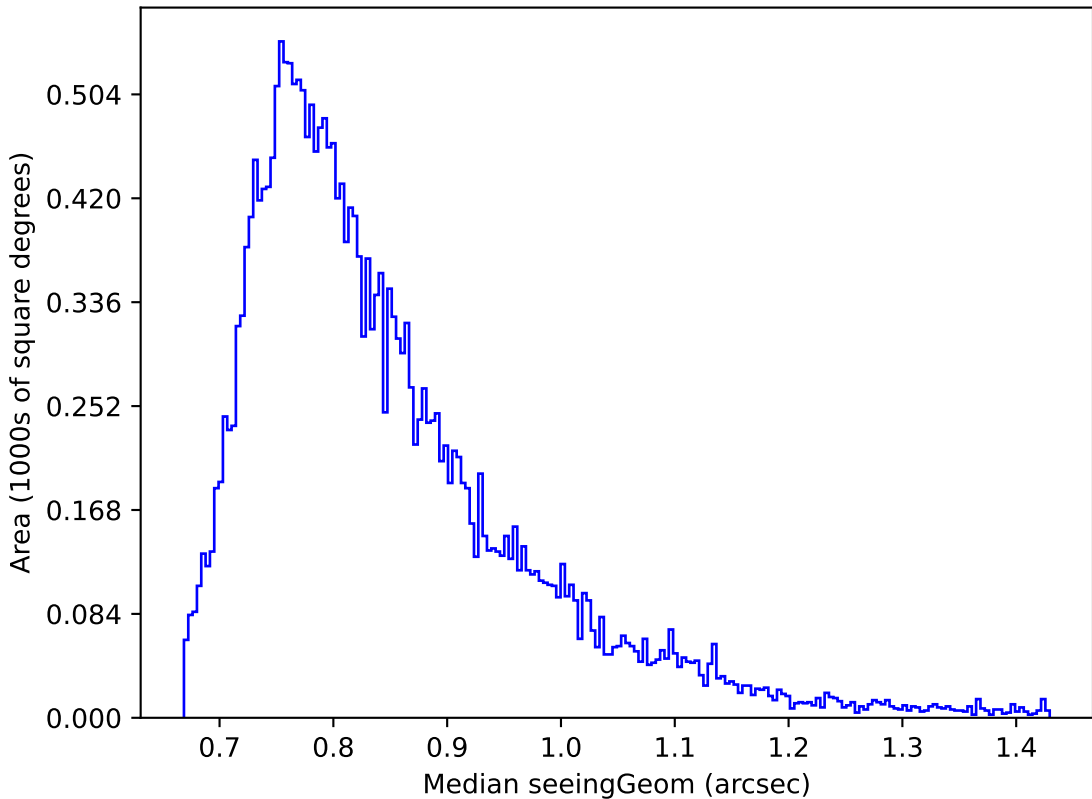
weather_cloudso16v3.4_10yrs Yr 1 i band: Median seeingGeom
