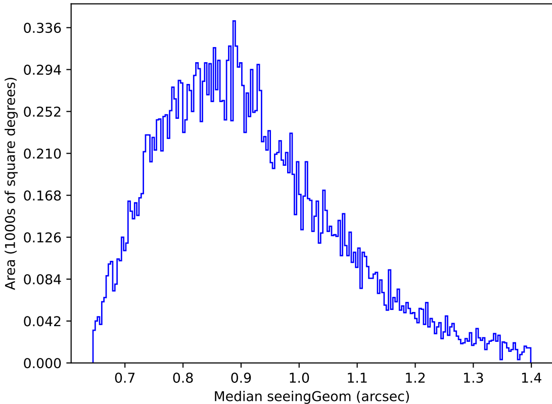
weather_cloudso16v3.4_10yrs Yr 1 g band: Median seeingGeom
