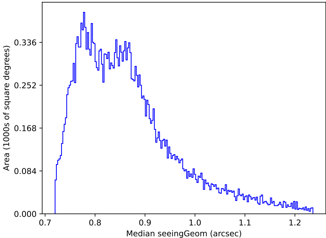
weather_cloudso16v3.4_10yrs Yr 1 all bands: Median seeingGeom
