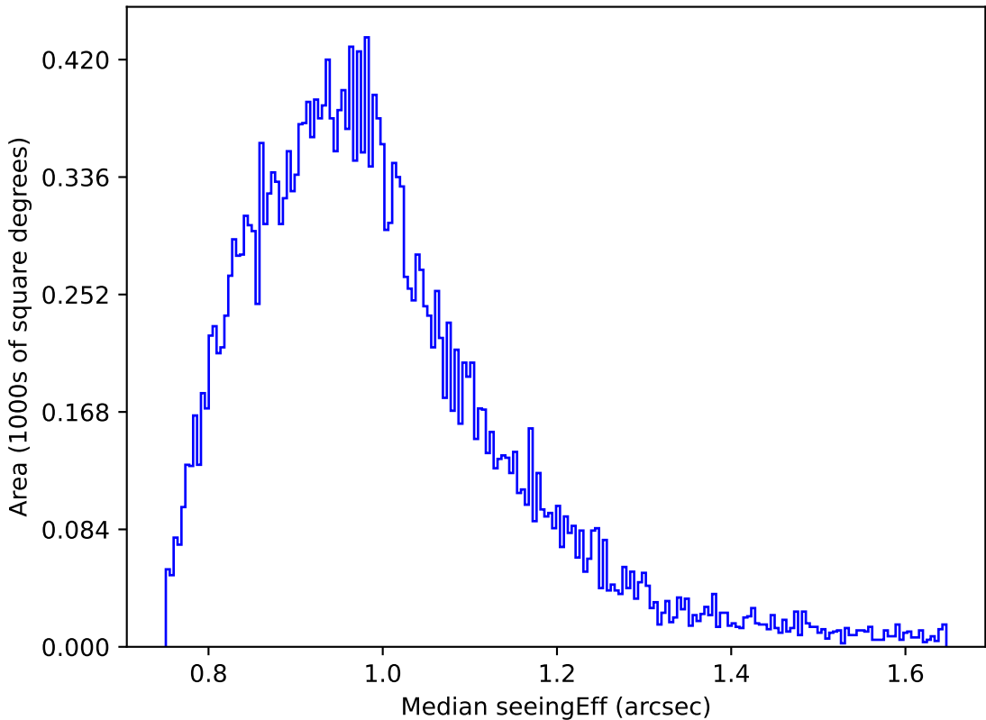
weather_cloudso16v3.4_10yrs Yr 1 z band: Median seeingEff
