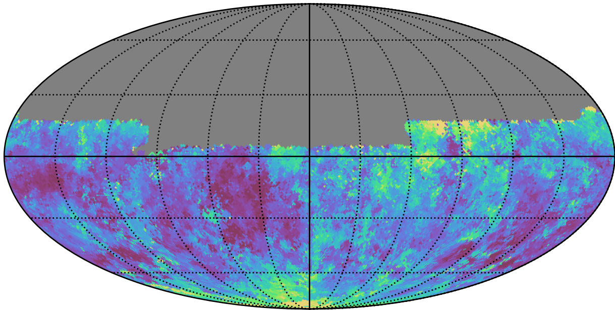
weather_cloudso16v3.4_10yrs Yr 1 y band: Median seeingEff
