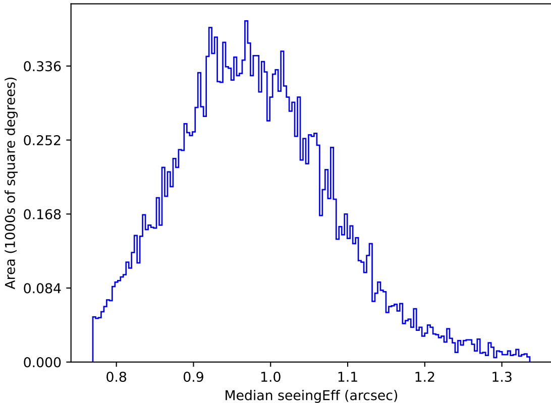
weather_cloudso16v3.4_10yrs Yr 1 y band: Median seeingEff
