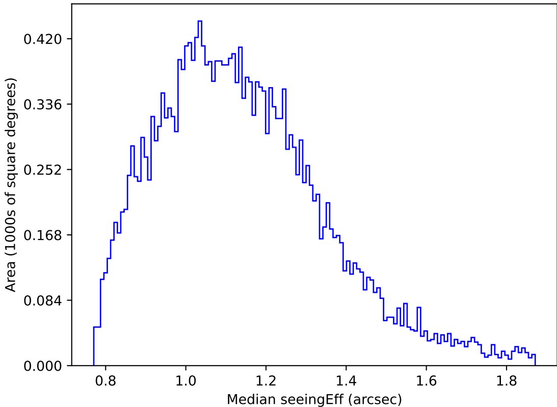
weather_cloudso16v3.4_10yrs Yr 1 u band: Median seeingEff
