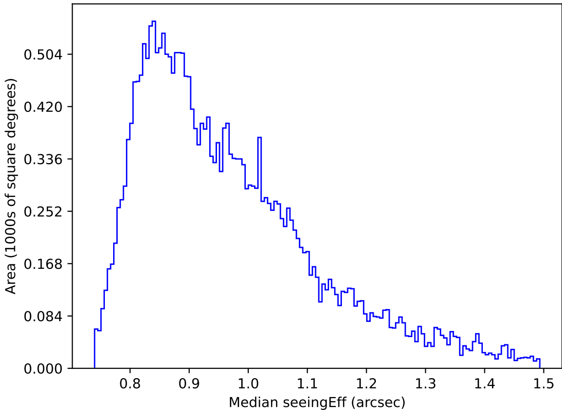
weather_cloudso16v3.4_10yrs Yr 1 r band: Median seeingEff
