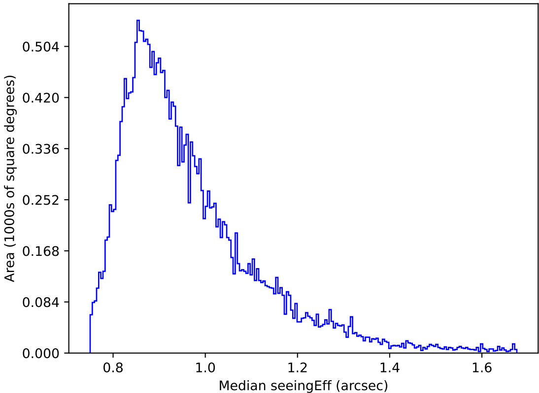
weather_cloudso16v3.4_10yrs Yr 1 i band: Median seeingEff
