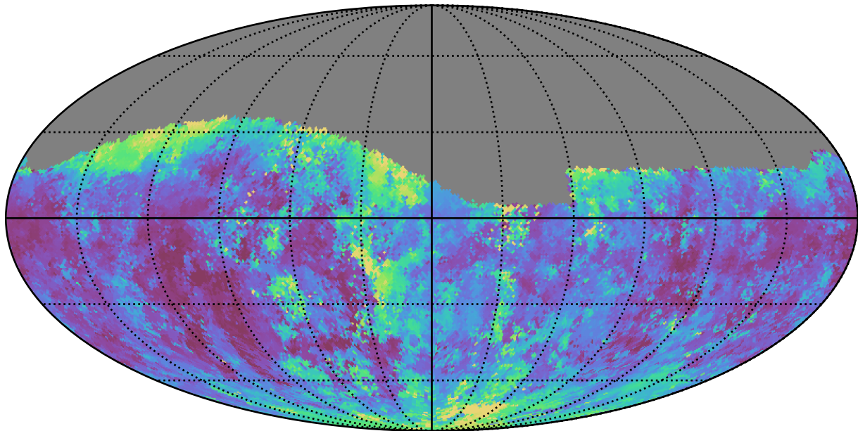
weather_cloudso16v3.4_10yrs Yr 1 g band: Median seeingEff
