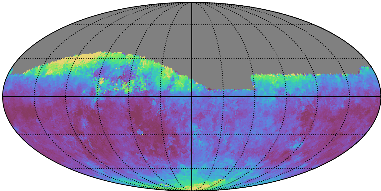
weather_cloudso16v3.4_10yrs Yr 1 all bands: Median seeingEff
